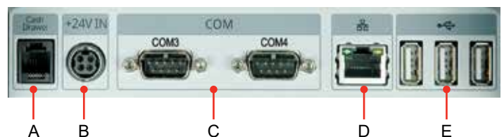
HM628N 10" Rugged Tablet shown with Optional Smart Dock.
